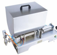
Paste filling machine
